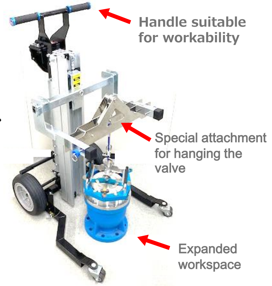
Original Lifter produced by Asada corp.
